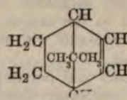
Bornylene.
